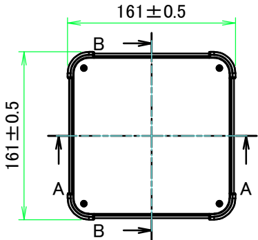
E view
