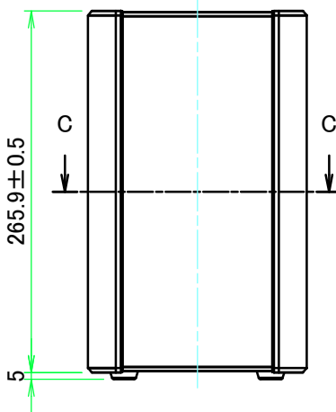
A view
